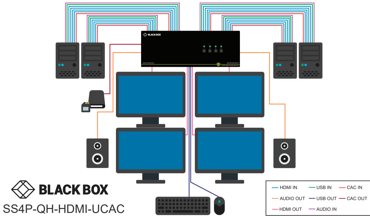
Figure 8-1 SS4P-QH-HDMI-UCAC Shown
