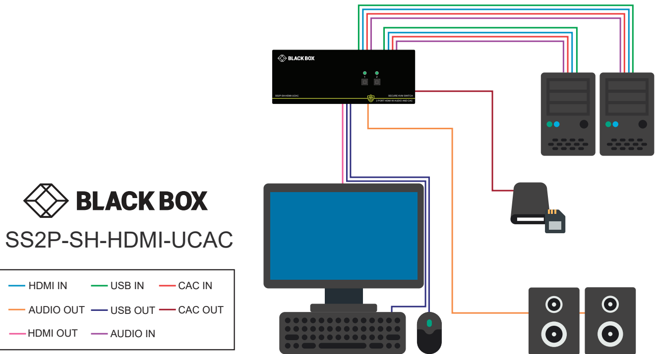
Figure 8-2 SS2P-SH-HDMI-UCAC Shown
